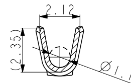
SECTION Y-Y
