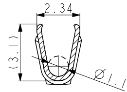
SECTION X-X
