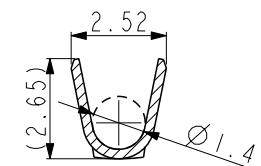
SECTION Z-Z
