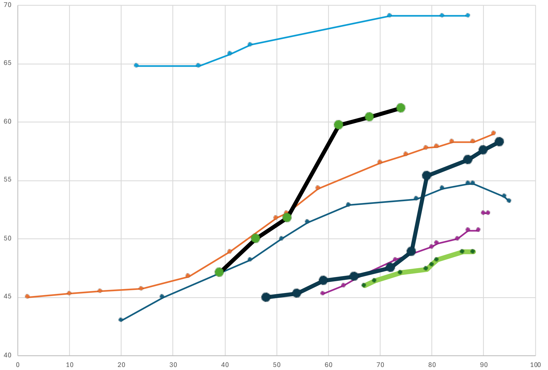
Battery Temp (F) as a Function of %SOC
